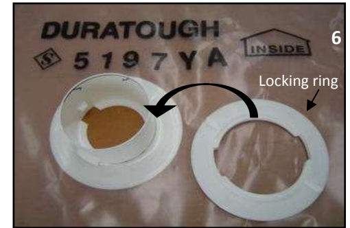
Position the locking ring over the flange base & by turning to lock it into place trapping the plastic film
